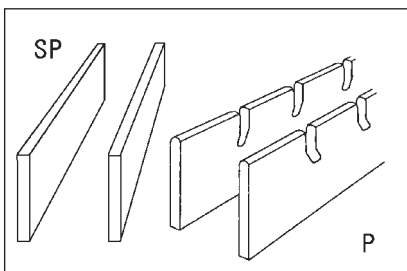
Bars bearing load lie parallel to each other between two grating supports
