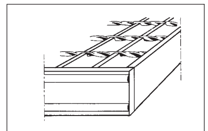
Bar or section to the edge of gratings, flush with the tops of bearing bars (in direction of bearing bar = binding along side; cross to bearing bar = cross binding).
