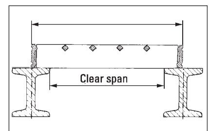
Distance between centre to centre of support. Clear span (effective span) is the clear distance between two supports.
