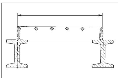
External distance of a metal grating in bearing bar direction. This size is termed length even if less than the width.
