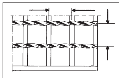
Distance between centre-to-centre of bearing bars and centre-to-centre of cross bars.
